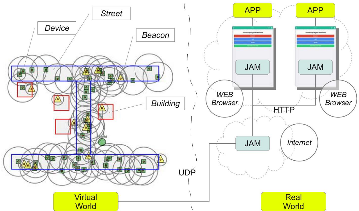
Figure 6. A demonstrator: An artificial street area consisting of street segments (blue rectangle) and buildings (red rectangles), beacons (yellow triangles), populated with stationary and mobile devices (green squares). The grey circles around beacons and nodes show the wireless communication range. Only overlapping circles connect.
