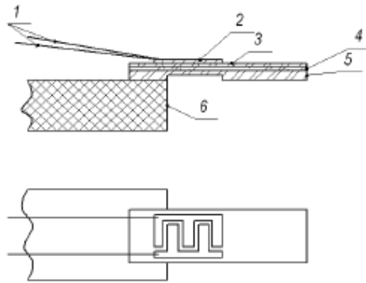
Figure 1. Schematic of laboratory sample of energy harvester : 1 - wires; 2 - contact pads; 3 - PZT film; 4 - silicon oxide; 5 - silicon.
