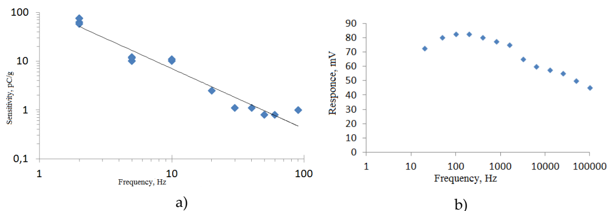
Figure 2. Dependence of energy harvester sensitivity on mechanical oscillations (a) and its response on the frequency of the electric field (b).
