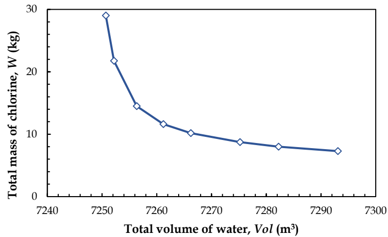
Figure 2. Pareto front of optimal solutions in the trade-off between total volume and total mass dosage
