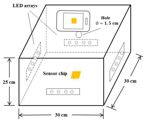
Figure 1. Diagram of the home-built photographic system for formaldehyde detection.
