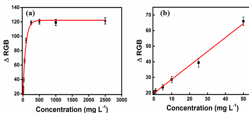
Figure 5. (a) Plot of \Delta RGB vs. formaldehyde concentration. (b) The relationship between \Delta RGB and formaldehyde concentration in the range of 0–50 mg L -1 .
