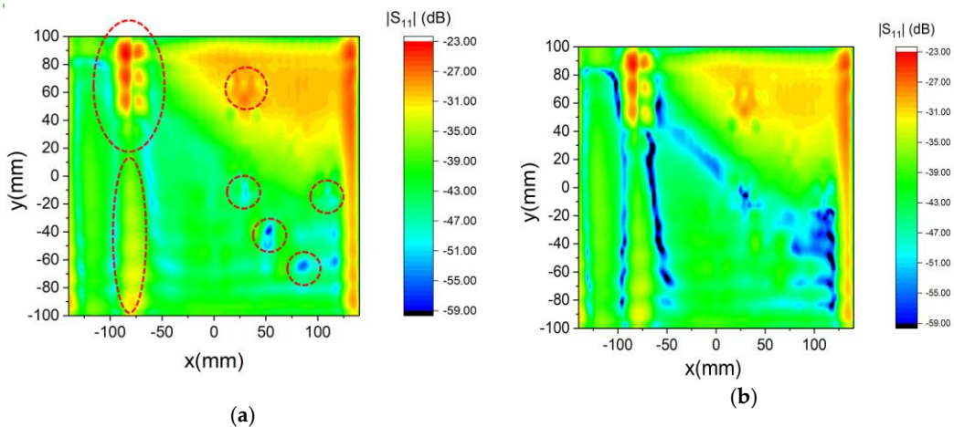
Figure 4. Reflected image represented by the |S_{11}| parameter magnitude at different frequencies: (a) 7.7773GHz. (b) 7.7776GHz. Encircled areas on Fig.4(a) show actual defects.
