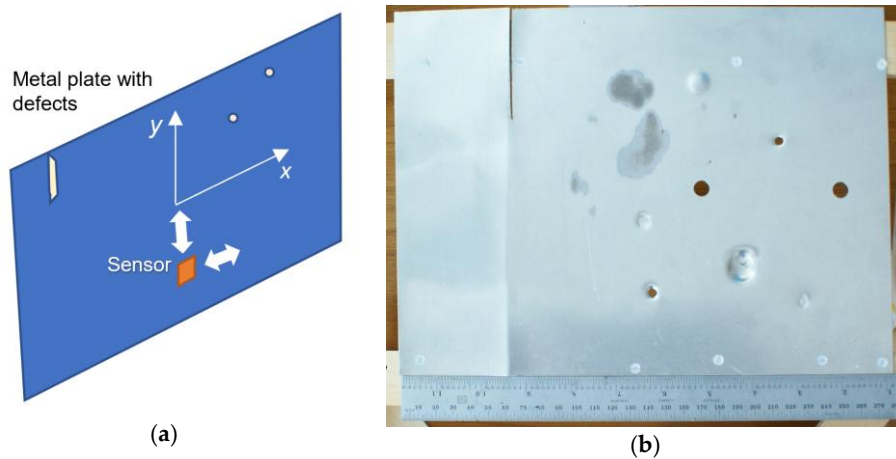
Figure 3. (a) Schematic geometry of scanning near field setup. The sensor’s standoff distance from the metal plate is 1mm-7mm. (b) Metal plate with various defects.
