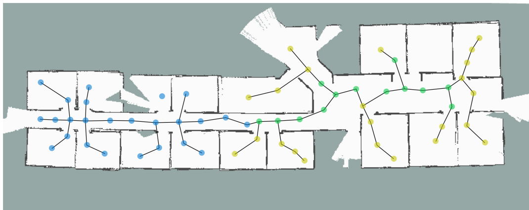
Figure 2. Multi-robot experiment. Robot A’s nodes are presented in yellow and Robot B’s in blue. The green nodes are the common or shared nodes between the two robots and the merged map is presented as grid map.
