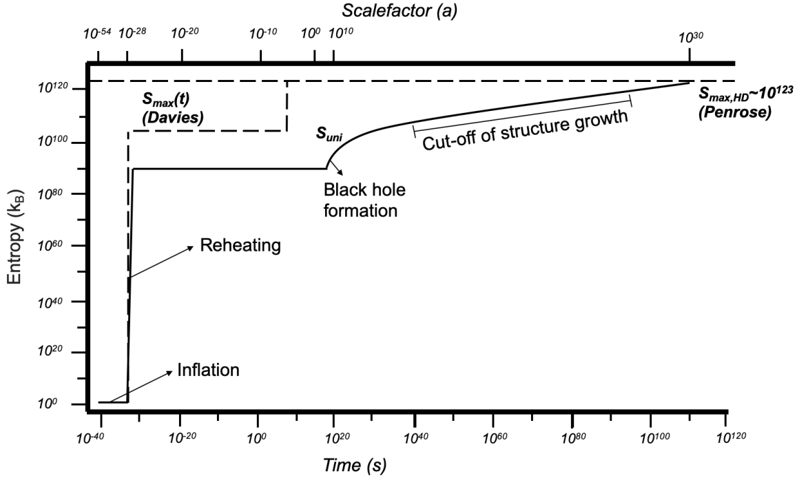
Figure 2 - The dashed lines refers to the competing models for maximum entropy. The maximum entropy achieved at heat death S_{max,HD} is a constant value at S \sim 10^{123}k . The time-dependent maximum S_{max}(t) as described by Davies [22] considers which processes at a given point in the evolution can contribute to entropy increase. It does not account for the rate at which these processes can increase entropy but does try to account for the total amount of entropy the new entropy-increasing processes could produce. The limits on the rate of entropy production will slow as the expansion of the universe prevents further accretion of mass onto supermassive black holes in the \Lambda -dominated era.
