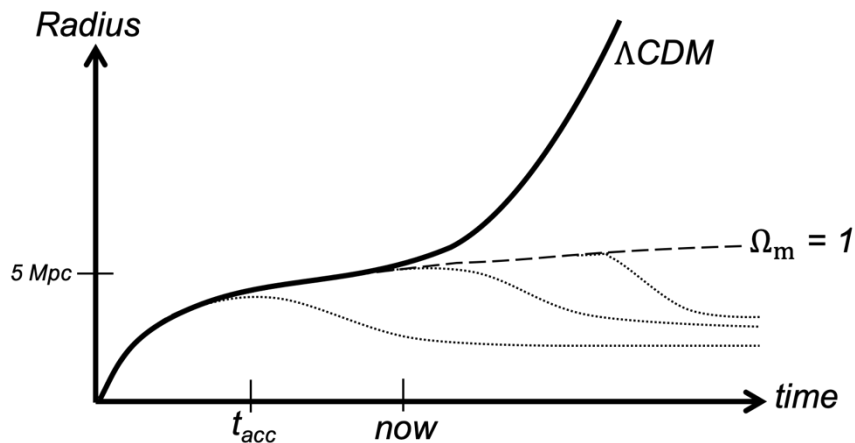
Figure 3 - Following the growth of size for a spherical distribution of matter. Dotted lines describe the virialization of structure by gravitational collapse. Dashed line: A flat \Omega_m = 1 universe in which structure formation does not turn off. Solid line: The consensus \Lambda - CDM universe in which structure formation turns off, with the largest objects on order of galaxy clusters \sim 5 Mpc, having already formed.
