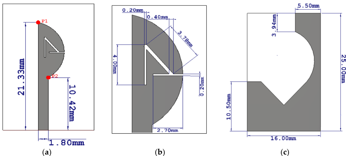
Figure 1. Ultra wideband band notch textile antenna: (a) front view, (b) Front view with details of slit size, and (c) Back view with showing ground plane size.
