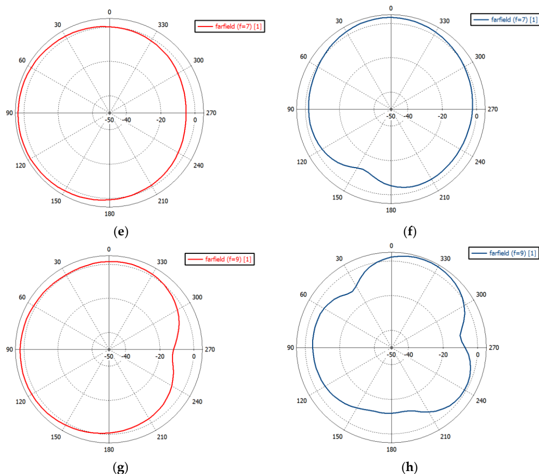
Figure 3. Radiation patterns of the antennas at different frequencies. (a) 3.5 GHz, XY Plane; (b) 3.5 GHz, XZ Plane; (c) 5.7 GHz, XY Plane; (d) 5.7 GHz, XZ Plane; (e) 7 GHz, XY Plane; (f) 7 GHz, XZ Plane; (g) 9 GHz, XY Plane; (h) 9 GHz, XZ Plane.
