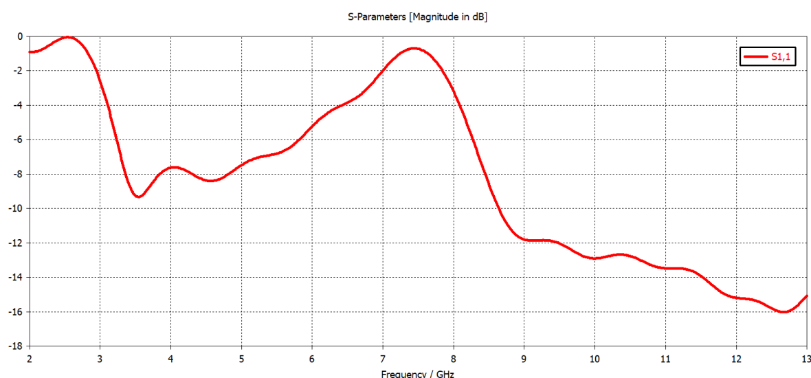
Figure 2. Return loss curve of the ultra-wideband (UWB) notch antenna.
