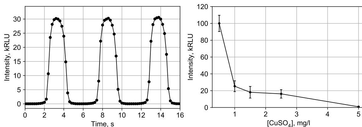
Figure 2. Signals from 3 droplets and dependence of luminescence intensity from \text{CuSO}_4 concentration
