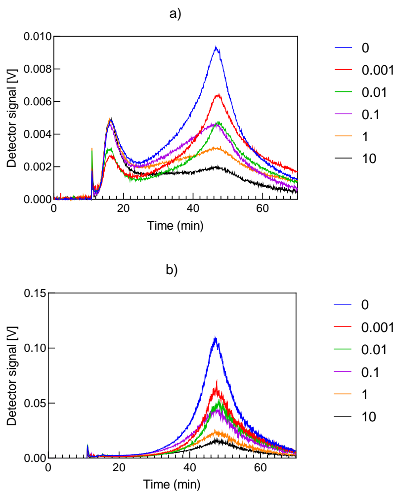
Figure 5. Aptamer-FB1-AuNP conjugate at different FB1 concentration upon addition of NaCl (0.2 M) detected by UV: 600 nm (a); and MALS: 28° (b) signals.
