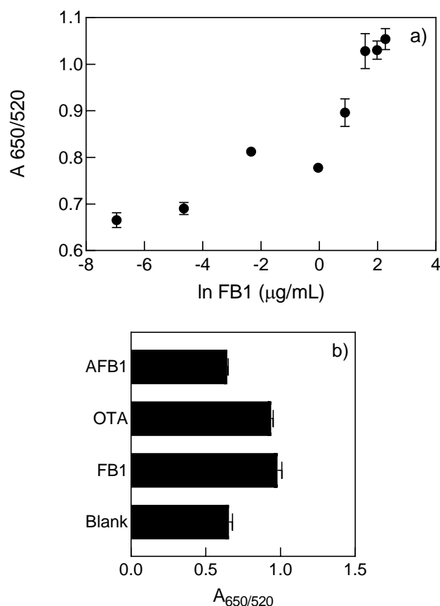
Figure 3. A 650/520 ratio of AuNP functionalized with a 40-nt aptamer previously incubated with FB1 in Tris HCl 14.06 mM pH 7.5 (Incubation: 60 min at 37 °C, Functionalization: 105 min at 20 °C, Aptamer:AuNP 500:1) after the addition of NaCl 0.4 M (a); specificity test after the incubation with buffer (blank), FB1, aflatoxin B1 (AFB1), and ochratoxin A(OTA) at a mycotoxin concentration of 13.8 µM (b).
