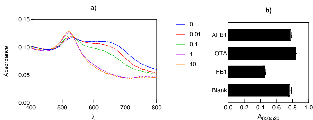
Figure 4. UV-VIS spectra of AuNP functionalized with a 96-nt aptamer previously incubated with FB1 (0-10 \mu\text{g/mL} ) in \text{MgCl}_2 1 mM (Binding: 30 min at 37 ^\circ\text{C} , Functionalization: 60 min at RT, Aptamer: AuNP 30:1) after the addition of \text{NaCl} 0.2 M (a); specificity test after the incubation with buffer (blank), or FB1, aflatoxin B1 (AFB1), and ochratoxin A(OTA) at a concentration of 1.38 \mu\text{M} (b).
