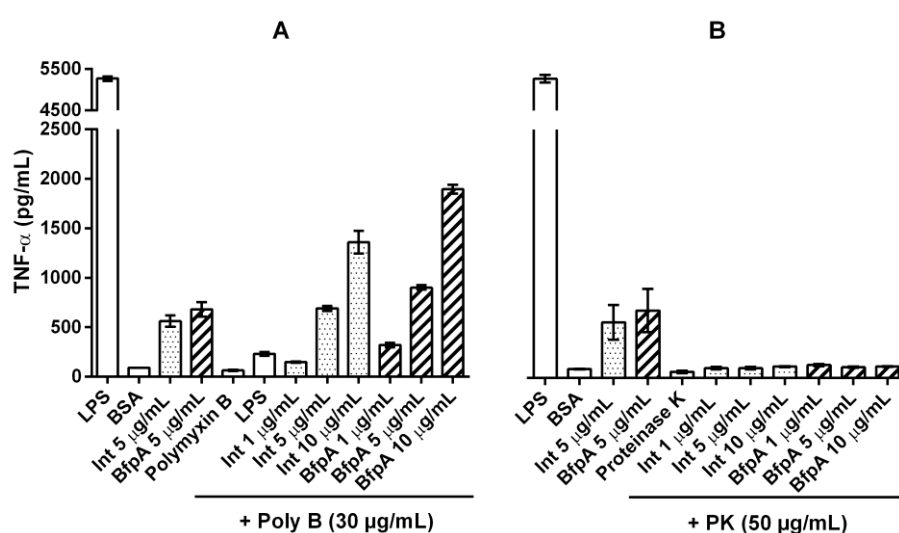
Figure 3. J774 cells ( 6 \times 10^5 cells) were stimulated with either intimin or BfpA pretreated with 30 µg/mL of polymyxin B (A) and 50 µg/mL of proteinase K (B) for 20 h. The supernatant was obtained to measure TNF- \alpha . The results are representative of the mean \pm SEM of two independent experiments, performed in triplicate.
