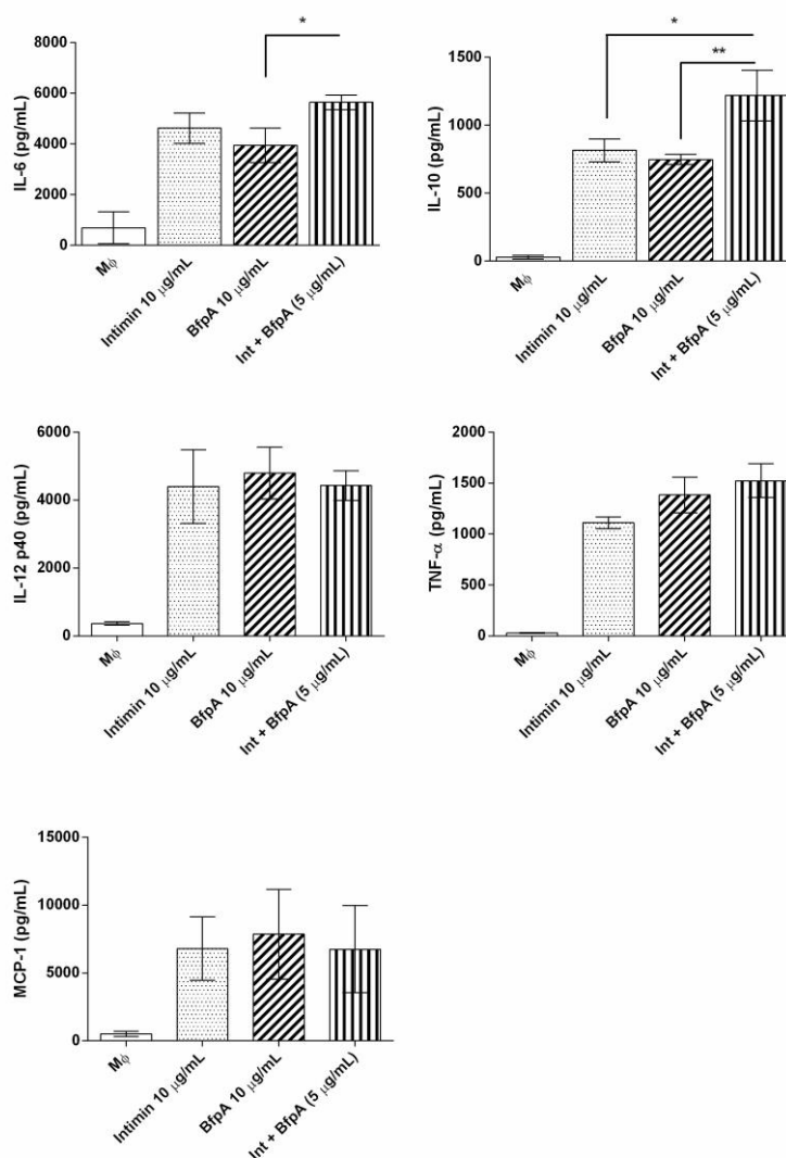
Figure 2. M \phi ( 6 \times 10^5 cells) were stimulated with the combination of intimin and BfpA (5 \mu\text{g/mL} and 5 \mu\text{g/mL} ). After 20 h the supernatant was obtained for cytokines and chemokine measurement. The results are representative of the mean \pm SEM of three independent experiments, performed in duplicate. The values * p < 0.05 and ** p < 0.001 were considered significant.
