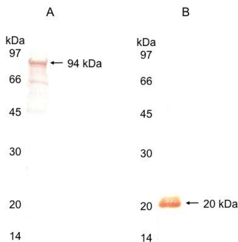
Figure S1. Expression of the proteins intimin \beta 3 and BfpA. Nitrocellulose membranes containing purified protein fractions of intimin \beta 3 (94 kDa) and BfpA (20 kDa) were incubated in the presence of rabbit specific IgG followed by goat anti-rabbit IgG peroxidase-conjugated. A: intimin \beta 3 protein; B: BfpA protein.
