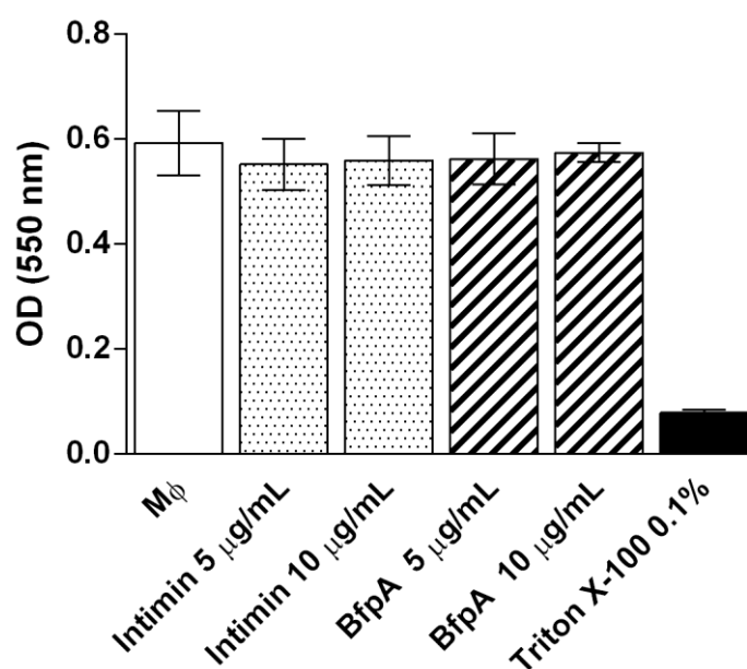
Figure S2. Cell viability of macrophages after treatment with intimin and BfpA. Mφ ( 6 \times 10^5 cells) were stimulated with intimin and BfpA (5 μg/mL and 10 μg/mL) for 20 hours. Cell viability was determined by the MTT assay. Triton X-100 (0.1%) was used as a cytotoxicity control. The results are representative of the
