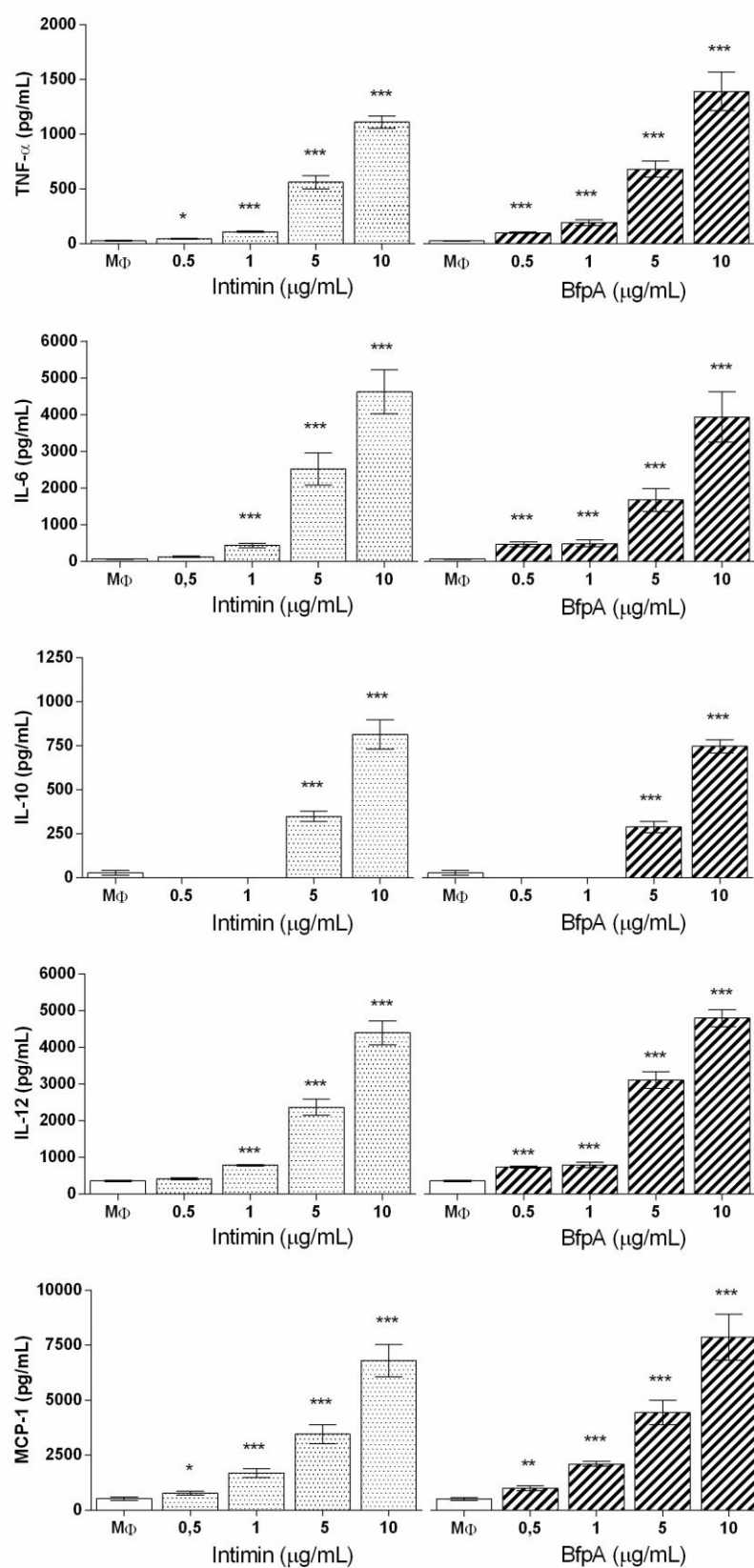
Figure 1. M \phi ( 6 \times 10^5 cells) were stimulated with 0.5 to 10 \mu g/mL of intimin or BfpA for 20 h. The synthesis of cytokines and chemokine was analysed in the culture supernatant by the ELISA assay. Data represent the mean \pm SEM of three independent experiments, performed in duplicate. The values * p < 0.05 , ** p < 0.001 or *** p < 0.0001 were considered significant.
