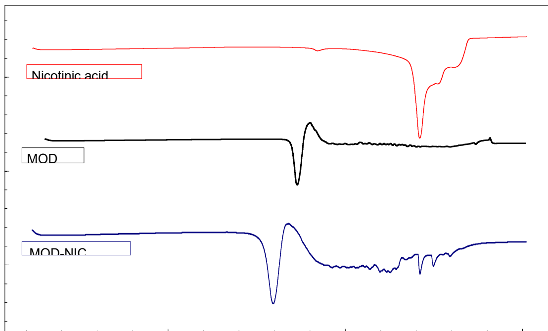
Figure 1: Overlay of DSC of modafinil, nicotinic acid, and modafinil-nicotinic acid cocrystals
