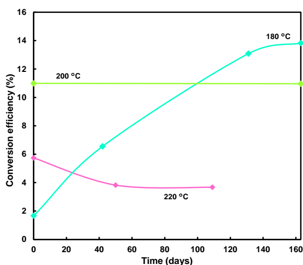
Figure 2. Changes of conversion efficiencies of \text{MA}_{0.64}\text{FA}_{0.31}\text{K}_{0.05}\text{PbI}_3 photovoltaic devices prepared at 180, 200, and 220\text{ }^\circ\text{C} .
