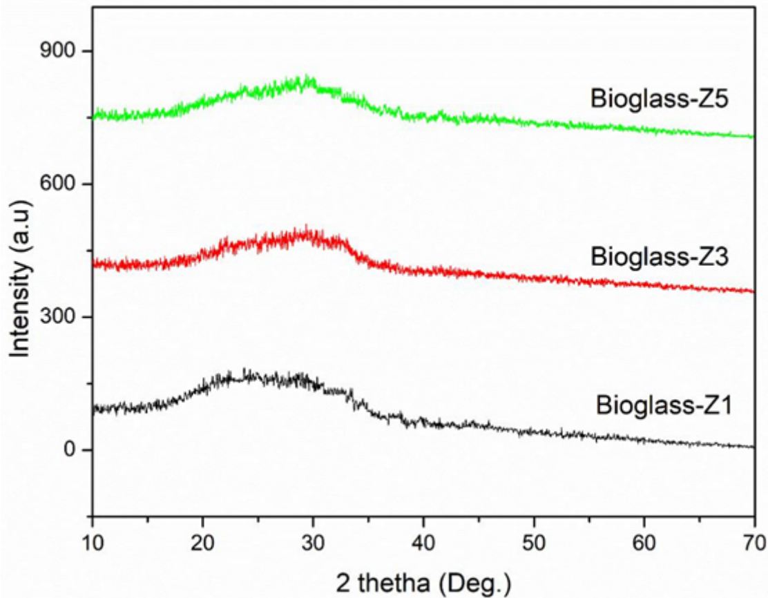
Figure 2. XRD patterns of bioactive glasses 70SiO_2-(30-x)CaO-xZnO (mol.%, x=1, 3, 5 ).
