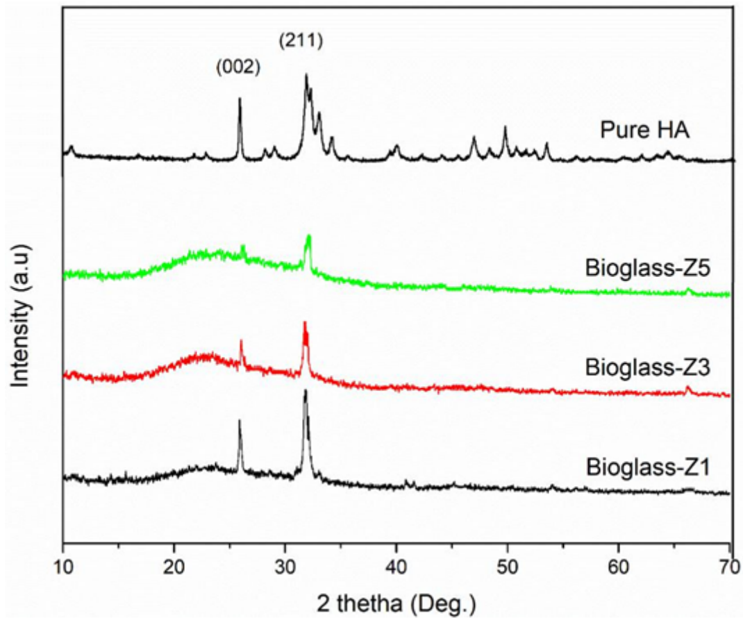
Figure 4. XRD patterns of bioactive glasses 70\text{SiO}_2-(30-x)\text{CaO}-x\text{ZnO} (mol.%, x=1, 3, 5 ).
