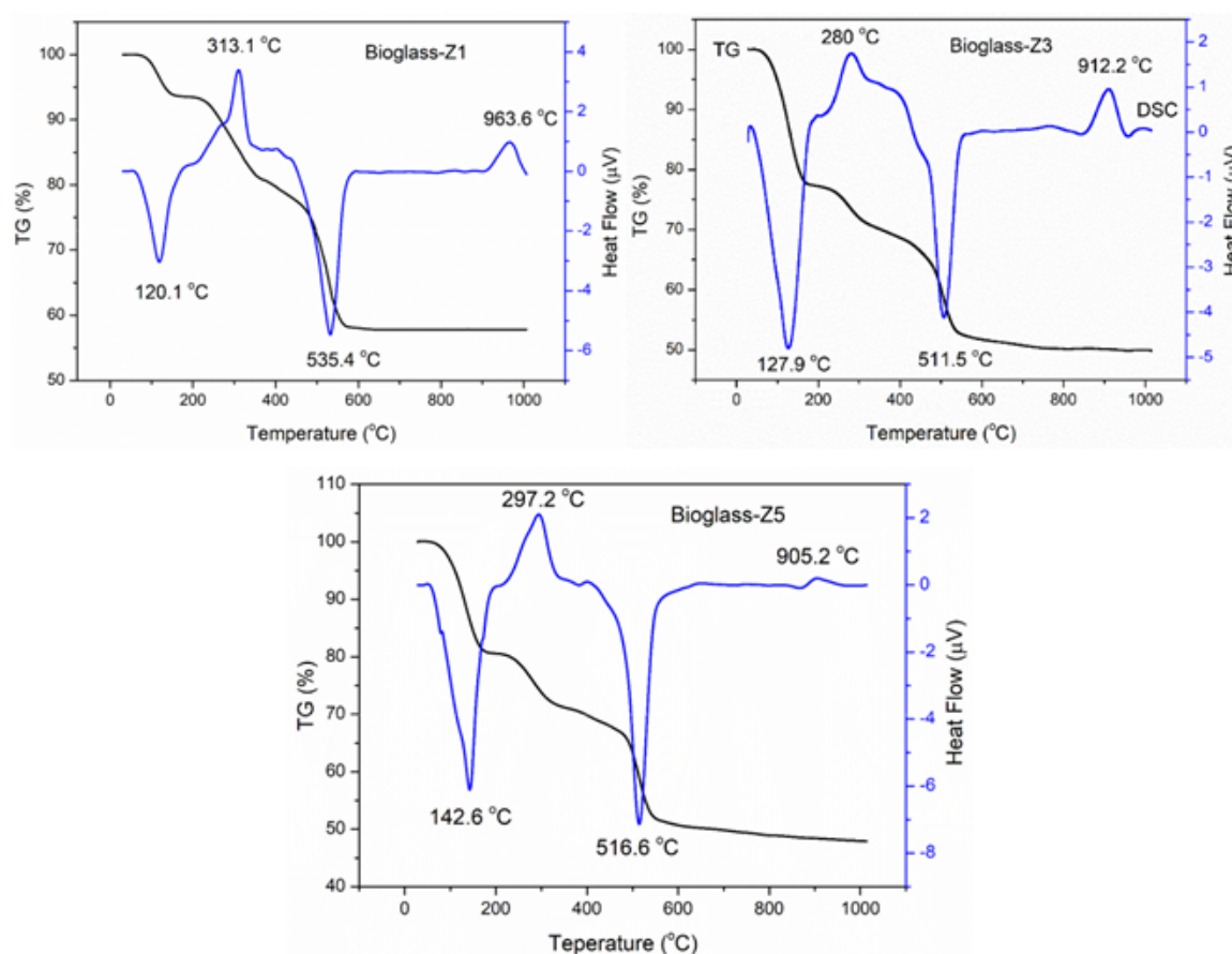
Figure 1. TG-DSC curves of bioactive glasses 70\text{SiO}_2-(30-x)\text{CaO}-x\text{ZnO} (mol.%, x=1, 3, 5 ).
