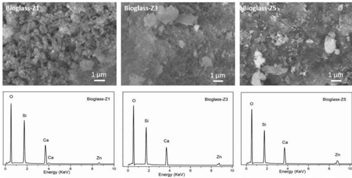
Figure 3. SEM-EDX analyses of bioactive glasses 70\text{SiO}_2-(30-x)\text{CaO}-x\text{ZnO} (mol.%, x=1, 3, 5 ).
