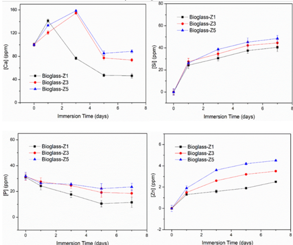
Figure 6. Ionic exchange between bioactive glasses 70\text{SiO}_2-(30-x)\text{CaO}-x\text{ZnO} (mol.%, x=1, 3, 5 ) and SBF solution.
