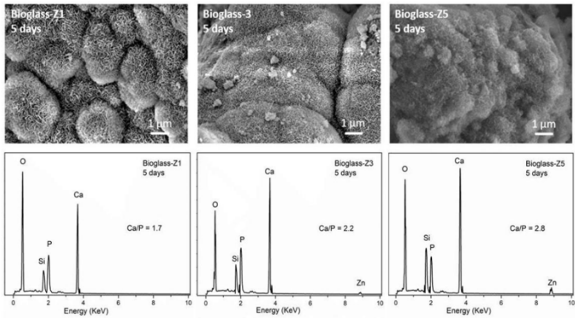
Figure 5. SEM-EDX analyses of bioactive glasses 70\text{SiO}_2-(30-x)\text{CaO}-x\text{ZnO} (mol.%, x=1, 3, 5 ) after 5 days in SBF solution.
