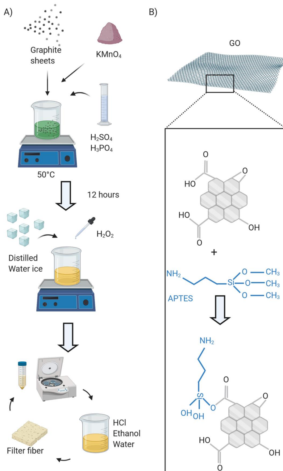
Figure 1. Scheme of the methodology conducted for: (A) Synthesis of GO: Oxidation of graphite sheets is carried out through the action of \text{KMnO}_4 , \text{H}_2\text{SO}_4 and \text{H}_3\text{PO}_4 . Once the oxidation step is quenched
