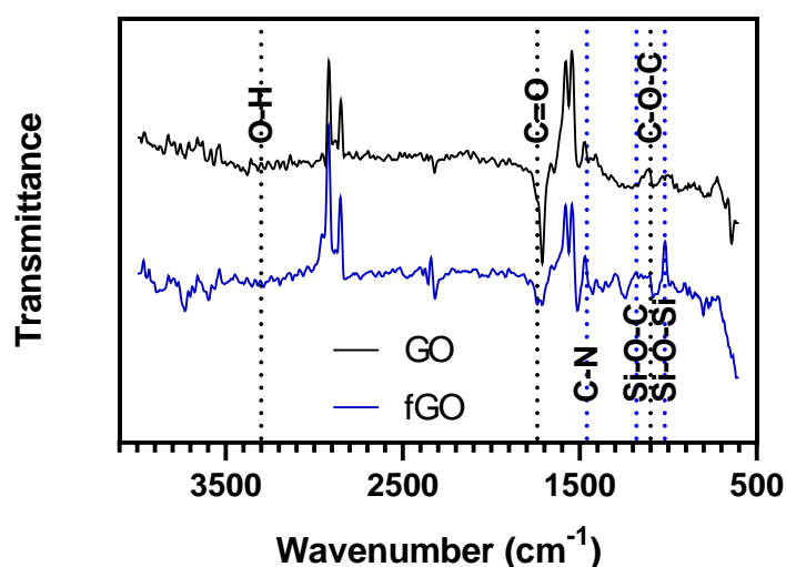
Figure 2. Infrared spectra for GO (black line) and fGO (blue line). After rendering amine groups on GO's surface, it was possible to observe characteristic peaks at 1020, 1180 and 1460 cm -1 attributed to expected bonds such as Si-O-Si, Si-O-C and C-N respectively.
