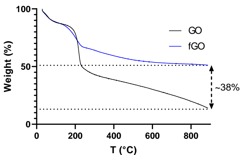
Figure 3. TGA profiles for GO (black line) and fGO (blue line). Within this temperature range GO lost over 85% of its mass, while fGO lost about 50% of its mass. This indicates that the functionalization process increased the density per weight unit of the functionalized GO. In addition, the difference between both curves gives a measurement of how efficient the functionalization process was.
