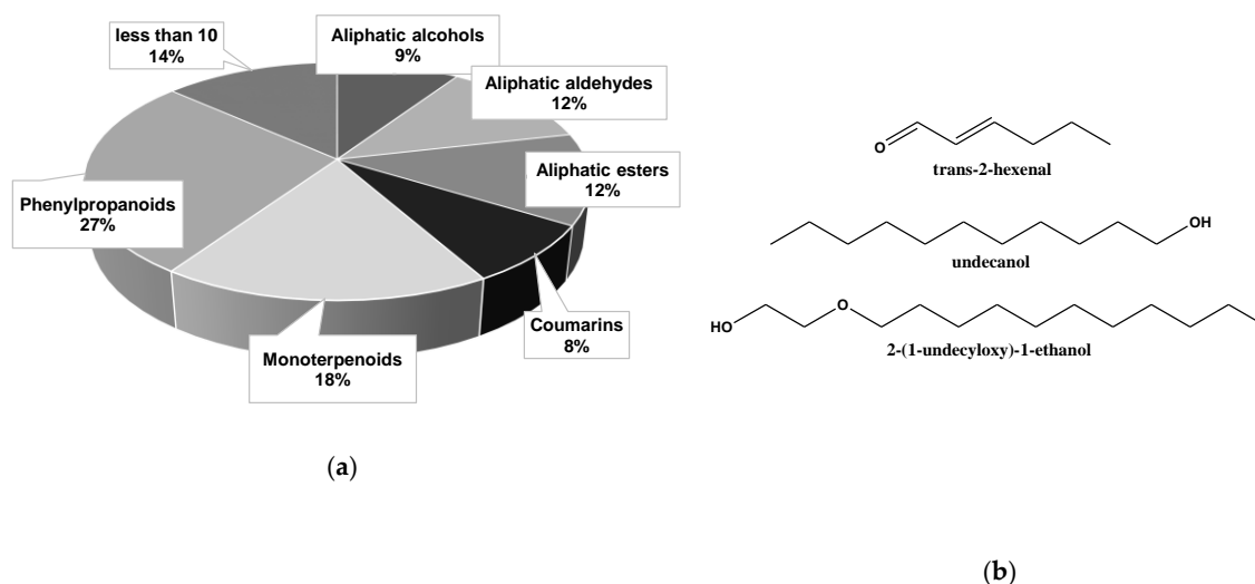
Figure 2. (a) Percentage of the main chemical groups of the volatile allelochemicals and derivatives reported against the PWN; “less than 10” includes classes with less than 10 instances. (b) The top 3 compounds with the lowest reported half maximal effective concentrations (EC 50 ).
