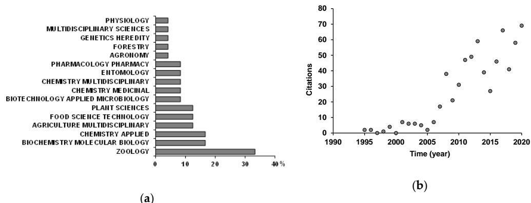
Figure 1. (a) Percentage of reports on the activity of volatile allelochemicals and derivatives against Bursaphelenchus xylophilus distributed by scientific journal areas and (b) yearly citation evolution of these reports.
