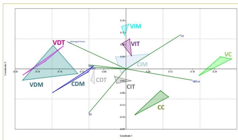
Figure 5. Results of the nMDS analysis is referred to all significant physical, chemical and biological soil parameters and damaged trees and summarize the complex situation. Difference tested among disturbed (Vallepietra Disturbed extracted by Tractor: VDT; Vallepietra Disturbed extracted by Mules: VDM; Camporotondo Disturbed extracted by Tractor: CDT; Camporotondo Disturbed extracted by Mules: CDM), undisturbed (Vallepietra Undisturbed extracted by Tractor: VIT; Vallepietra Undisturbed extracted by Mules: VIM; Camporotondo Undisturbed extracted by Tractor: CIT; Camporotondo Undisturbed extracted by Mules: CIM) and control (Vallepietra Control: VC; Camporotondo Control: CC), for the two mechanization levels in the two areas.
