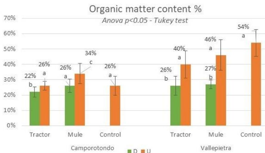
Figure 3. Results of the ANOVA and Tukey test for Organic matter content (OM), difference tested among disturbed (D), undisturbed (U) and control soil, for the two mechanization levels. Different letters after means within each mechanization level indicate significant differences by Tukey test ( p < 0.05 ).
