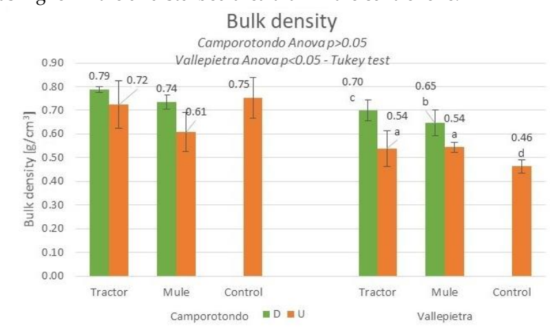
Figure 1. Results of the ANOVA and Tukey test for Bulk density, difference tested among disturbed (D), undisturbed (U) and control soil, for the two mechanization levels. Different letters after means within each mechanization level indicate significant differences by Tukey test ( p < 0.05 ).
