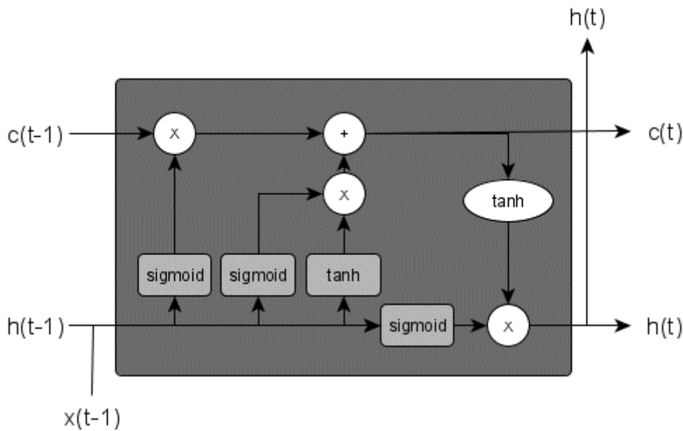
Figure 2. Structure of a LSTM memory cell. The 'x' represents an input, 'h' is a hidden state, 'c' is a cell state, sigmoid and tanh represent the respective activation function.
