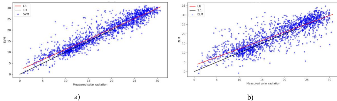
Figure 3. Linear regression of a) SVM solar radiation estimates using 48T+48RH+Ra (best model with the best configuration) and b) ELM using 48T (worst model and configuration).
