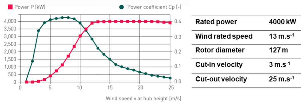
Figure 1. Power curve (in kW) of the selected wind turbine (4 MW E-126 EP3, ENERCON) for wind speed ranging from 0 to over the cut-out velocity (25 ms -1 ). Note the rated (maximum) power of 4000 kW, wind rated speed of 13 ms -1 (outlined by the vertical dotted line), rotor diameter of 127 m and cut-in velocity of 3 ms -1 . Adapted from: [20, 30].
