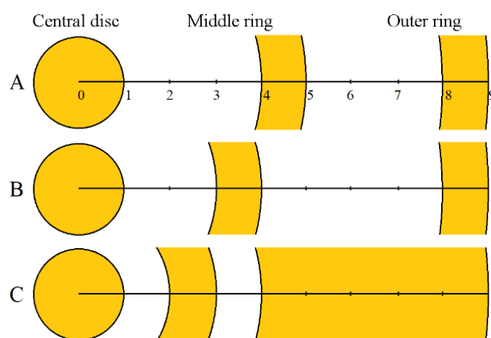
Figure 1. Finite dimensions models of three tripolar concentric ring electrode configurations including: (A) constant inter-ring distances configuration, (B) linearly increasing inter-ring distances configuration, and (C) optimal configuration with respect to the accuracy of Laplacian estimation.
