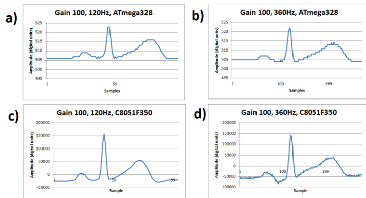
Figure 4. ECG signal from human volunteer A, (lead I). (a) Gain 100x, sample rate 120 Hz on ATmega328 microcontroller, (b) Gain 100x, sample rate 360 Hz on ATmega328 microcontroller, (c) Gain 100x, sample rate 120 Hz on C8051F350 microcontroller, (d) Gain 100x, sample rate 360 Hz on C8051F350 microcontroller.
