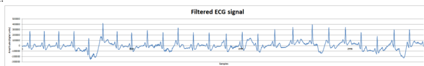
Figure 8. ECG signal from human volunteer B (lead DII). Filtered ECG signal with a second order Butterworth filter to reduce motion artifacts.
