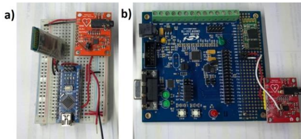
Figure 2. (a) Low-resolution ECG system with Arduino platform (ATmega328). (b) High-resolution system for ECG monitoring with Silicon LABS platform (C8051F350). In both cases, the Sparkfun AD8232 module with minor modifications was used for the analog stage.
