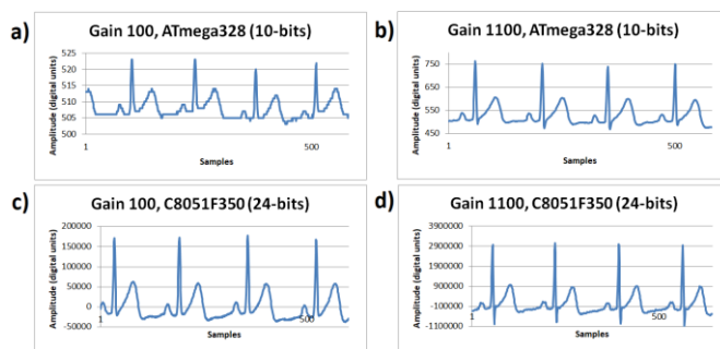
Figure 5. ECG signals sampled at 180 Hz rate from human volunteer A on resting state (lead I). (a) Gain 100x, ATmega328 (10-bits) with 100x gain. (b) ATmega328 (10-bits) with 1100x gain. (c) C8051F350 (24-bits) with 100x gain. (d) C8051F350 (24-bits) with 1100x gain.
