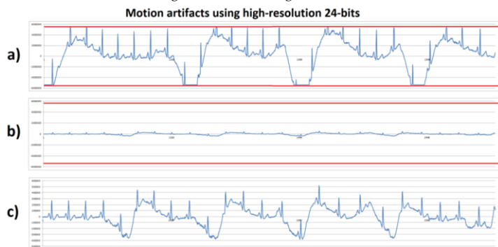
Figure 7. ECG signals from human volunteer B (lead DII) at stationary gait with a fast sudden movement using high-resolution 24-bits platform. (a) Motion artifact causing saturation limits
