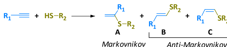
Scheme 1. Schematic representation of alkyne hydrothiolation.
