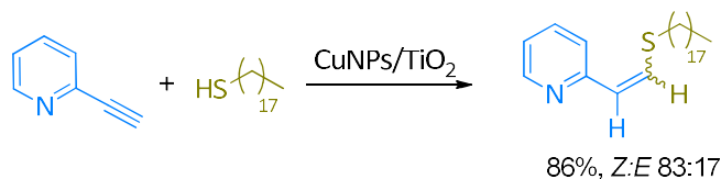
Scheme 2. Reaction between 2-ethynylpyridine and 1-octadecanethiol.
