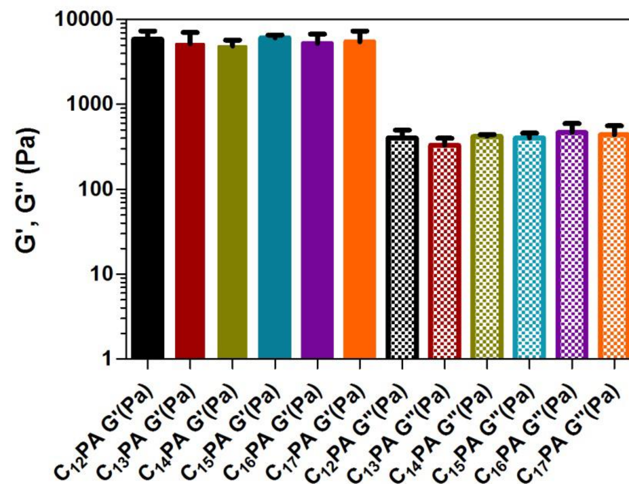
Fig. 4. Oscillatory rheology data of viscoelastic (G' >> G'') PA hydrogels.
