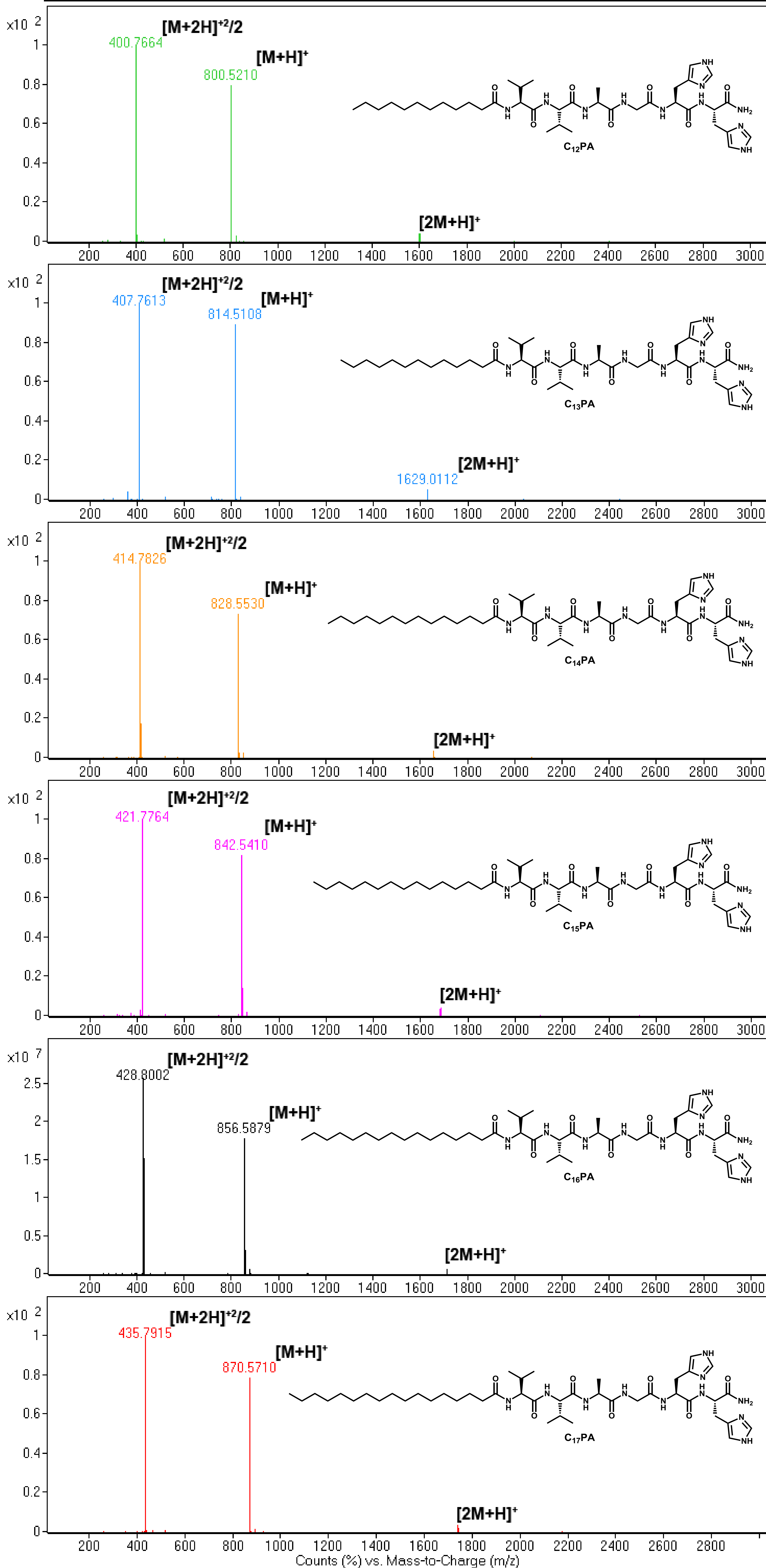
Fig.1. Molecular structures and mass spectra of PAs.
