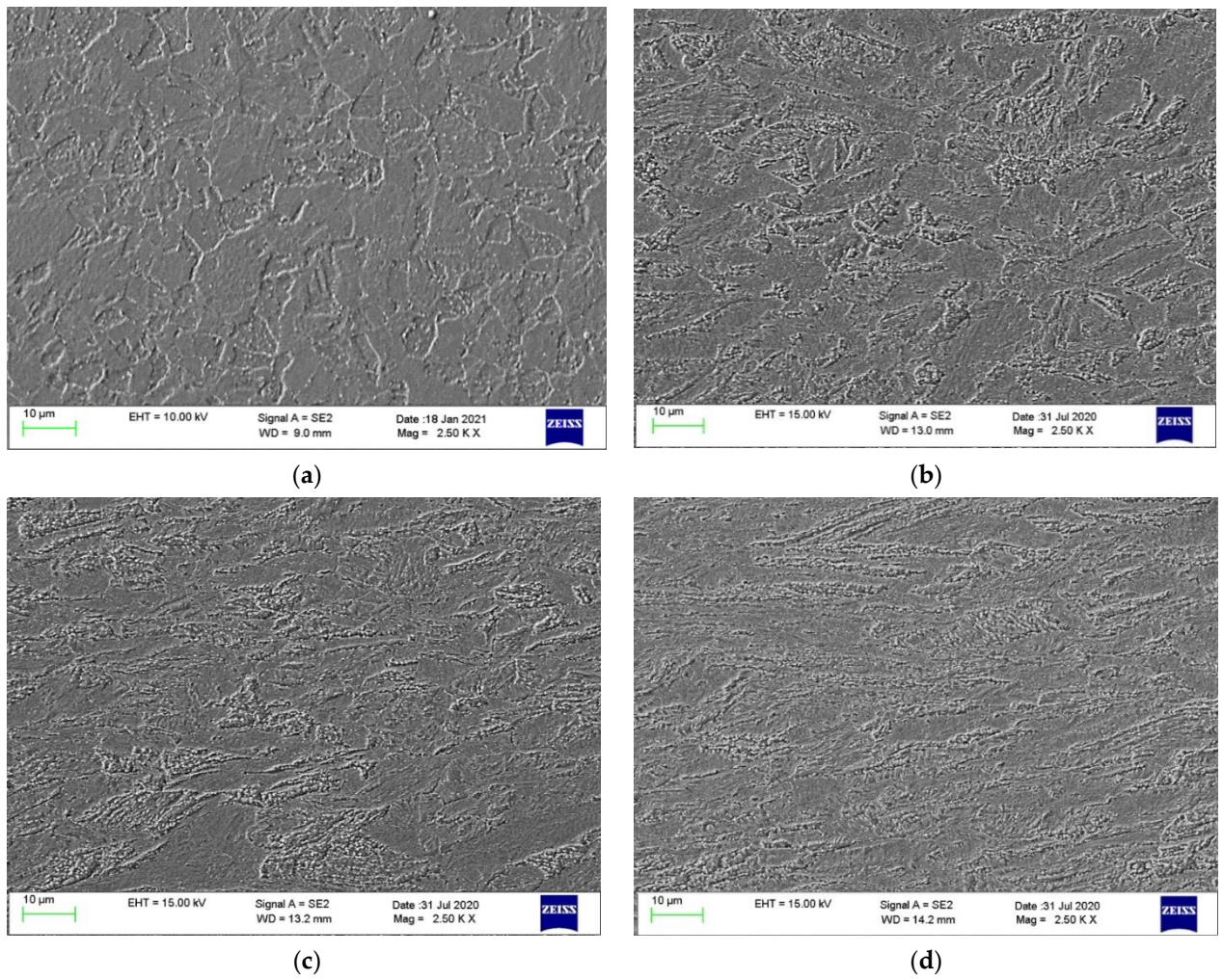
Figure 1. SEM images of (a) standard EUROFER97 state, (b) cold rolled EUROFER97 steel with CR: 30%, (c) cold rolled EUROFER97 steel with CR: 40% and (d) cold rolled EUROFER97 steel with CR: 50%.
