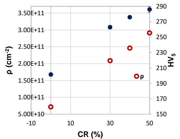
Figure 3. Effect of CR on Vickers hardness (HV 5 ) and dislocation density calculated by Williamson-Smallman relation (1) of EUROFER97 steel.
