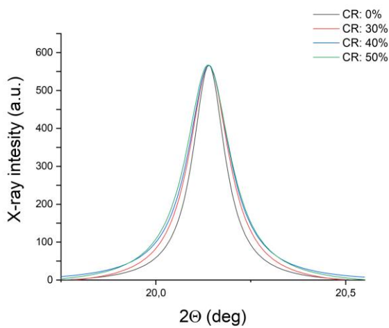
Figure 2. (a) Effect of the cold rolling process on the line shape of {100} X-Ray diffraction peak, of EUROFER97 steel.
