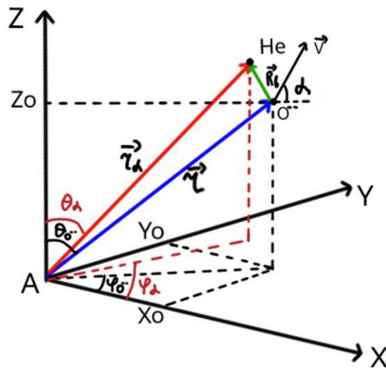
Figure 2. Coordinate system OHe–nucleus
