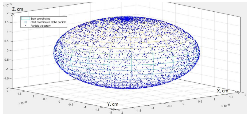
Figure 1. The density of the distribution of the coordinates of the \alpha -particle in the orbit corresponding to the ground state of the system
