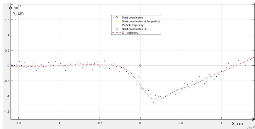
Figure 4. The trajectory of \alpha -particle and the O^{--} in the XY plane
