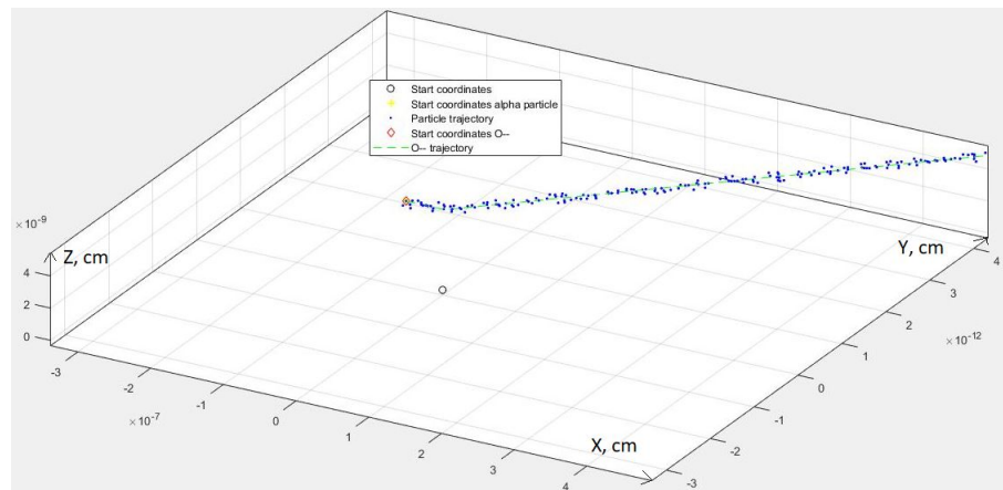
Figure 3. \alpha -particle and particle O^{--} trajectories
