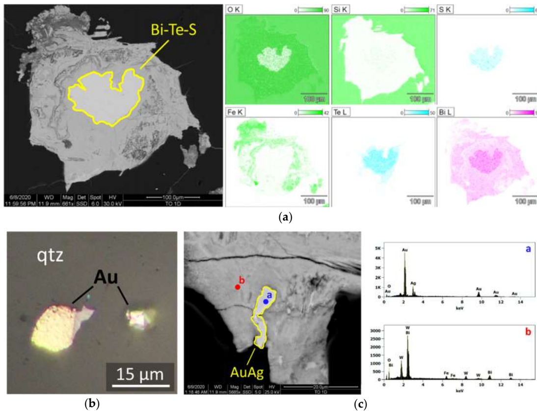
Figure 5. Bi-Te-Au mineralization from the Togoro wolframite veins: (a) Bi-sulfotelluride grain surrounded by bismite alteration (TO-1) (b) visible \mu\text{m} -scale gold grains enclosed in quartz (TO-1, 50x); (c) SEM-EDS spot analysis showing electrum (AuAg) grains, point a, enclosed in a Bi-tungstate, point b (TO-1).
