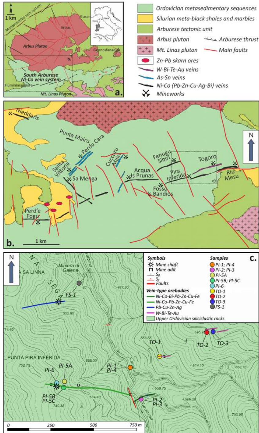
Figure 1. Geological sketch of the South Arburese area: (a) large-scale geological sketch showing the spatial relationships between the Arbus (304 Ma) and Linas plutons (289 Ma) and the orebodies (mod. after Moroni et al., 2019); (b) detail of the different vein-type orebodies of the area, including Ni-Co five-element type, As-Sn and W veins (mod. after Moroni et al, 2019); (c) small-scale geological sketch of the study area showing the location of the Pira Inferida five-elements type and Togoro W-Bi-Te-Au veins and the sampling sites.
