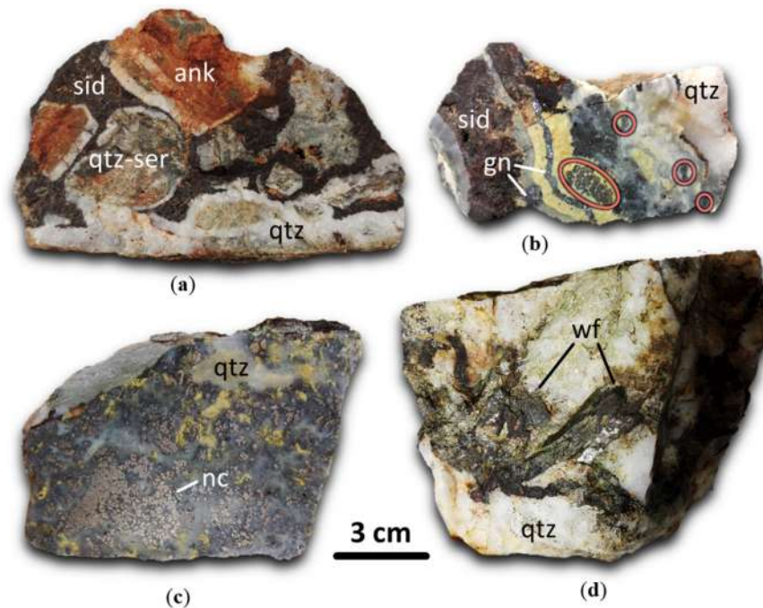
Figure 2. Hand specimens from the five-element veins at Pira Inferida and from the Togoro wolframite-bearing veins: (a) typical brecciated textures of the quartz and carbonate (siderite-ankerite) gangue (Pira Inferida, PI-1); (b) Bi and Ni-Co arsenide-sulfarsenide nests (in red) and thin galena veins in the siderite-quartz matrix (Pira Inferida, PI-5); (c) niccolite aggregates in the quartz matrix (Pira Inferida, PI-2); (d) idiomorphic wolframite crystals up to 6 cm in length in quartz gangue (Togoro, TO-2).
